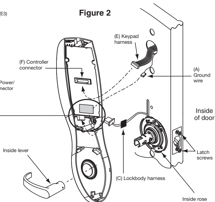
Ribbon Cable Orientation: Install with cable exiting DOWN, as shown.
